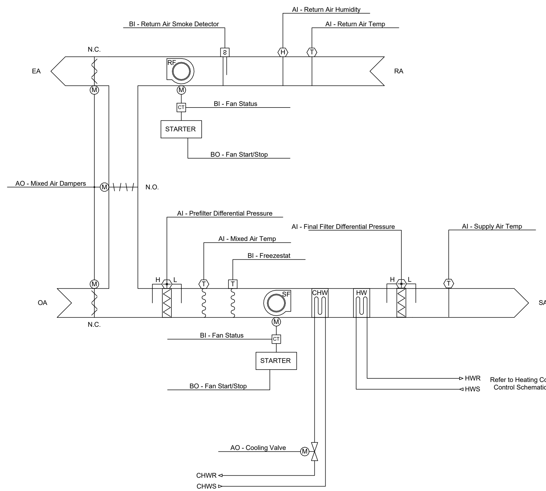
AHU-3 (BASEMENT) CONTROL SCHEMATIC (CONSTANT FLOW) SCALE: N.T.S.
