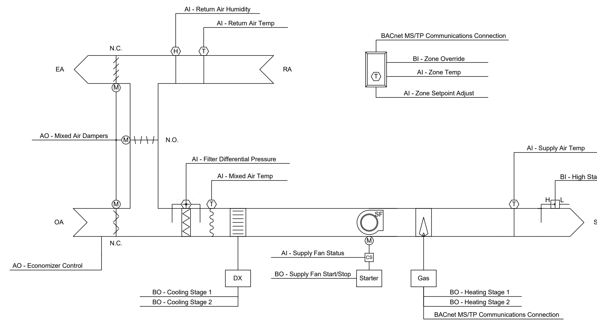
AHU-5 (FITNESS ROOM) CONTROL SCHEMATIC (CONSTANT FLOW) SCALE: N.T.S.
