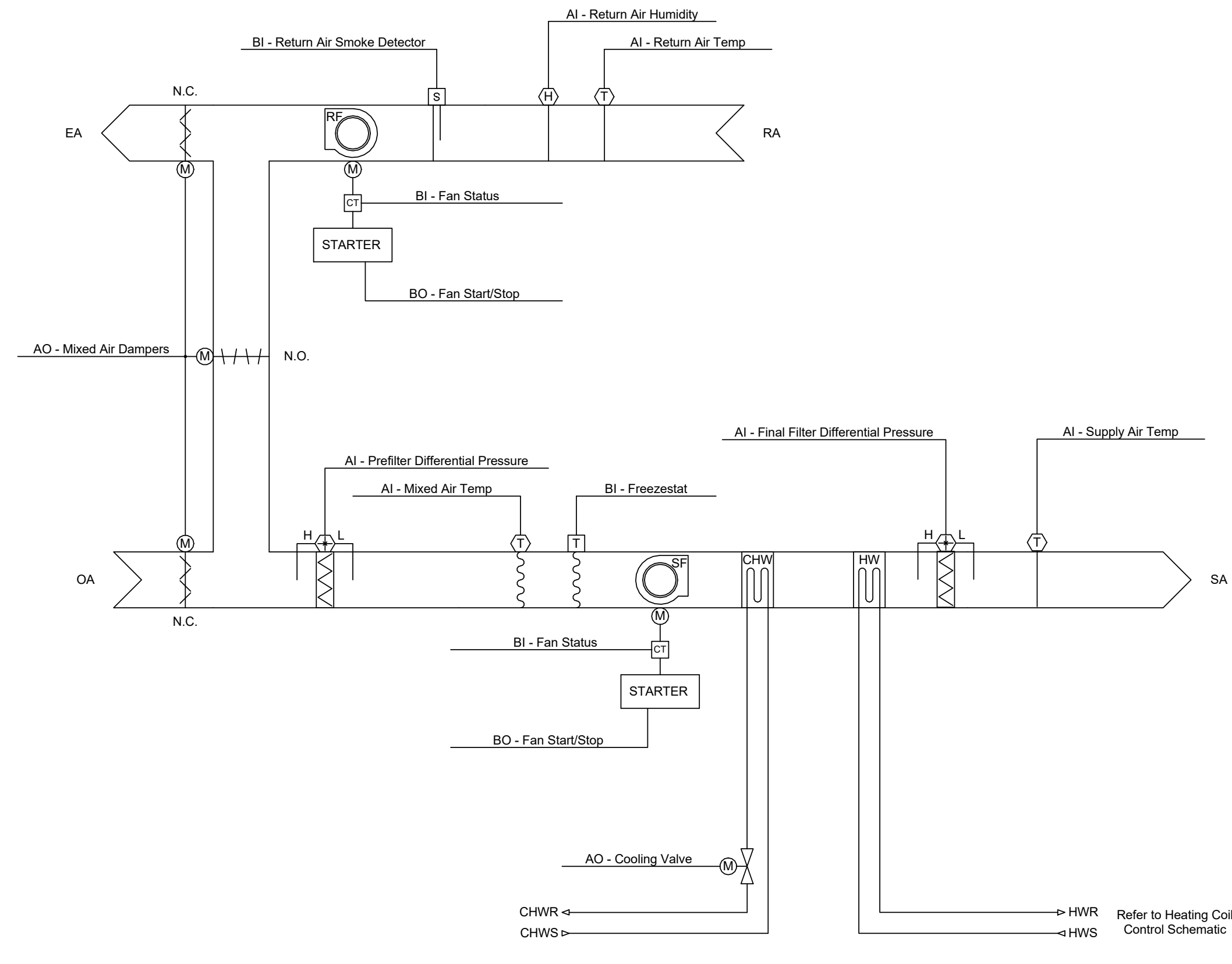
AHU-2 (LOBBY) CONTROL SCHEMATIC (CONSTANT FLOW) SCALE: N.T.S.
